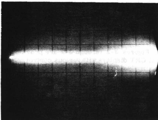
Figure 3-4. Single-shot trace bloom caused by INTENSITY and or PERSISTENCE set too high
